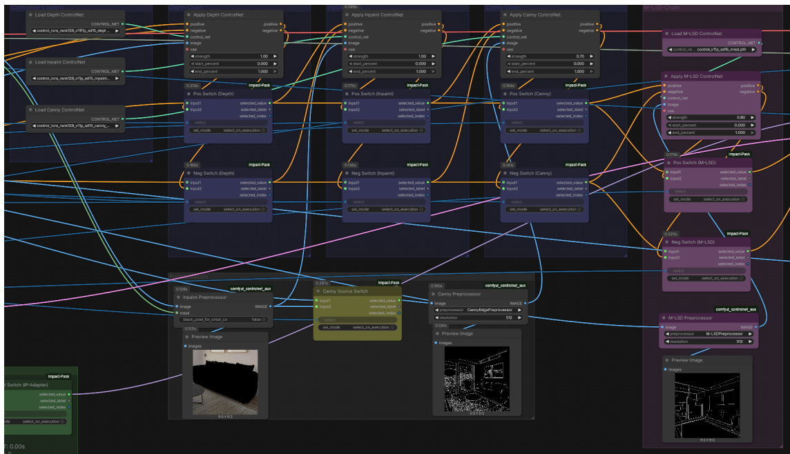
Figure 4.20: Style Injection Block: IPAdapter encodes reference product features and injects them into the diffusion latent space.
