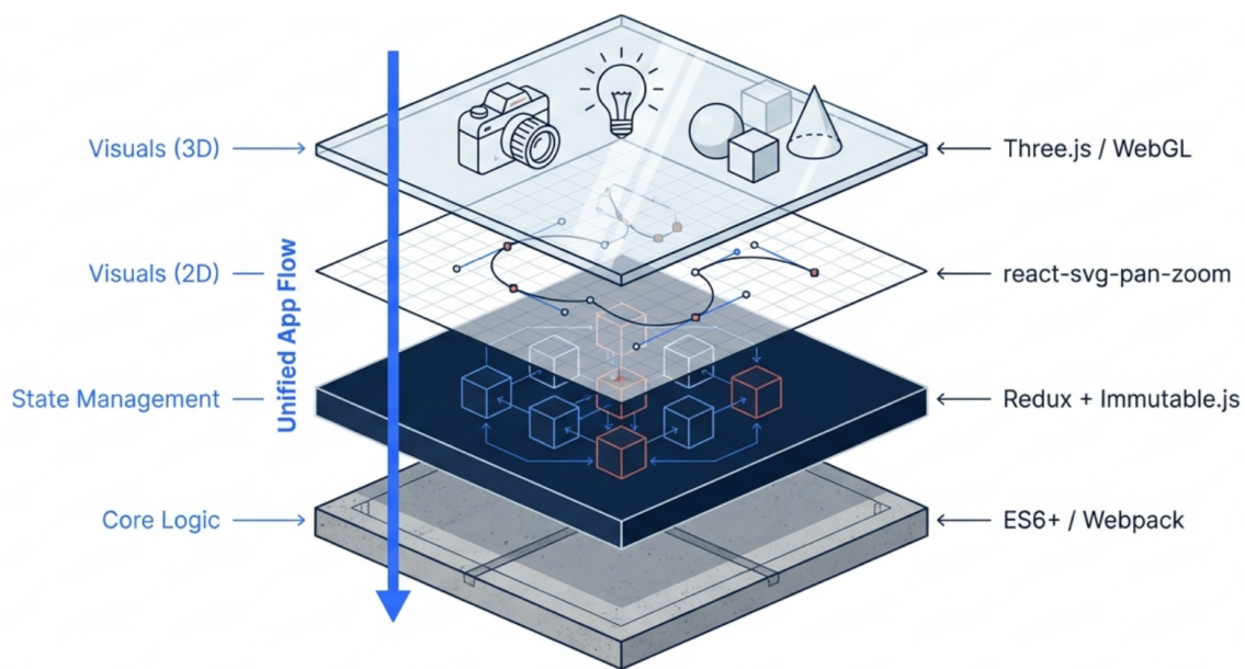
Figure 4.38: Floor Planner Technical Stack: Multi-layered architecture with Three.js for 3D rendering, React for UI components, and Redux for state management. The unified app flow connects Core Logic, State Management, 2D Visuals, and 3D Visuals layers.
