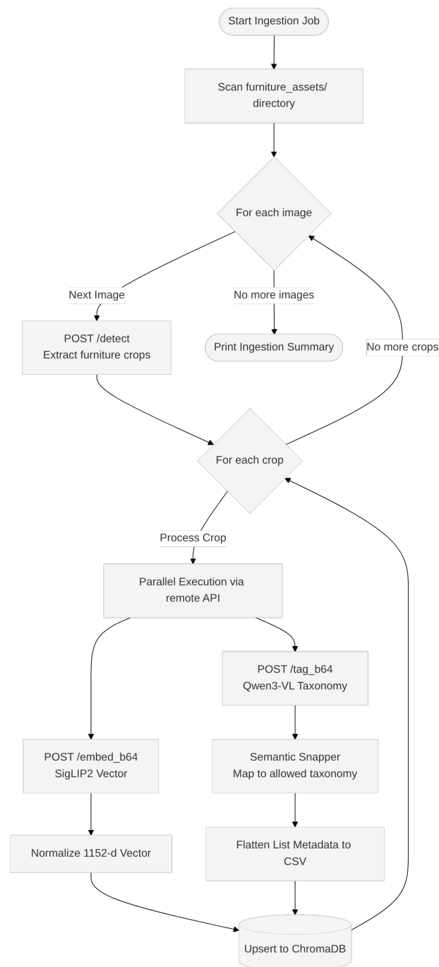
Figure 4.6: Offline Ingestion Pipeline: Catalog images are scanned, furniture crops are detected, parallel embedding and tagging are performed, metadata is normalized via the semantic snapper, and results are upserted into ChromaDB.
