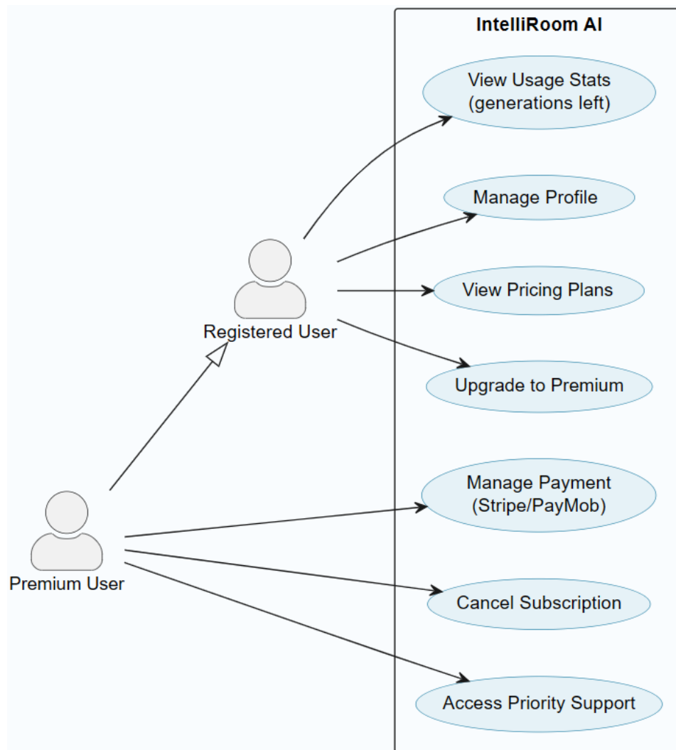
Figure 3.4: Use Case Diagram: AI Design Generation Process
