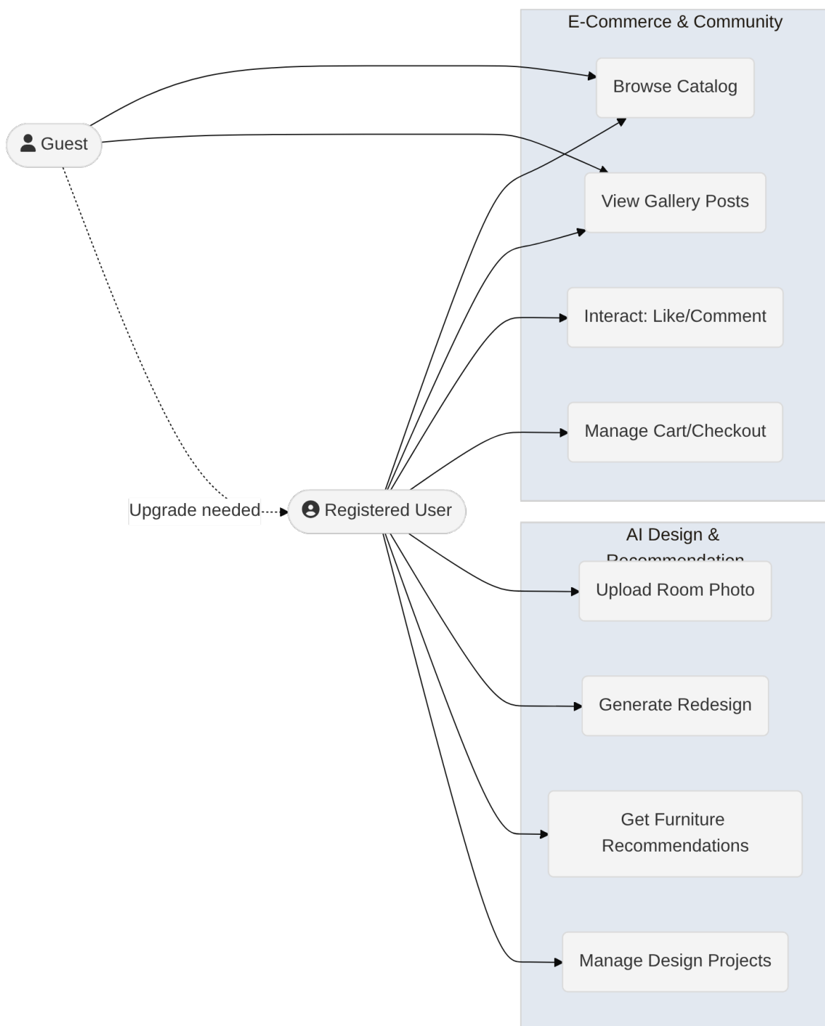
Figure 3.1: System Use Case Overview: Guest and Registered User roles mapped to E-Commerce, Community, and AI Design capabilities.
