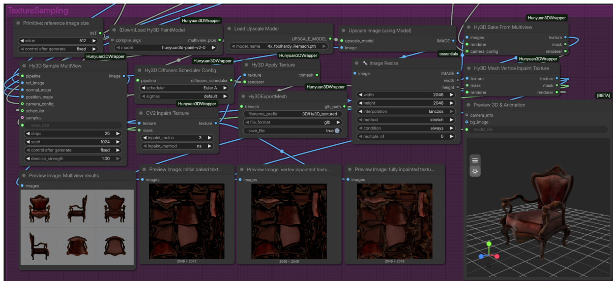
Figure 4.10: 3D Reconstruction Pipeline Part 3: UV mapping, inpainting, upscaling, and final .GLB export.
