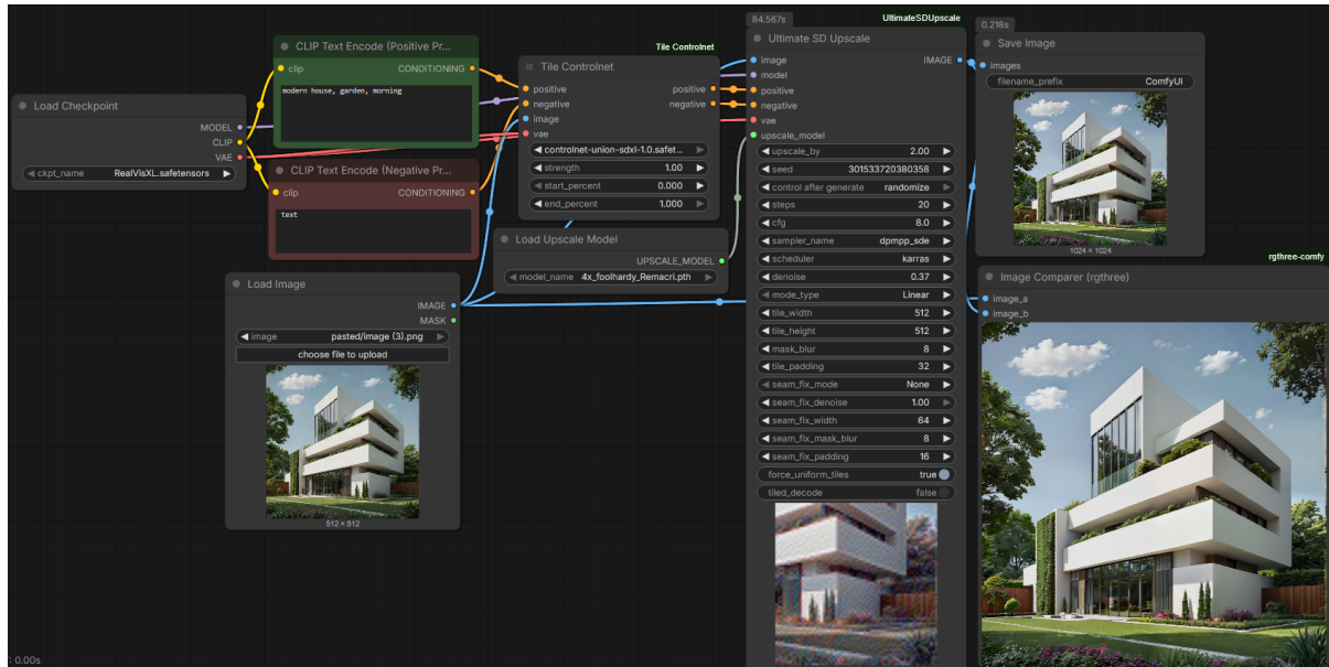
Figure 4.15: Ultimate Upscale Workflow: Tiled diffusion with 4x_foolhardy_Remacri upscaler and Tile ControlNet for high-resolution exports.
