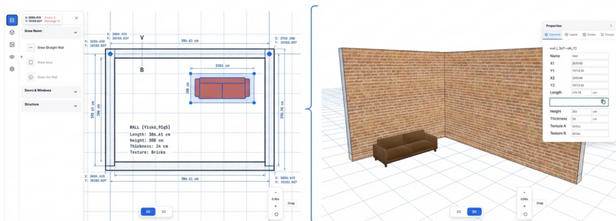
Figure 4.43: Integrated 2D/3D Workflow: Synchronized editing with simultaneous 2D blueprint and 3D preview. Changes in either view update the opposite view in real-time. Right panel provides parametric property editing with instant visual feedback.
