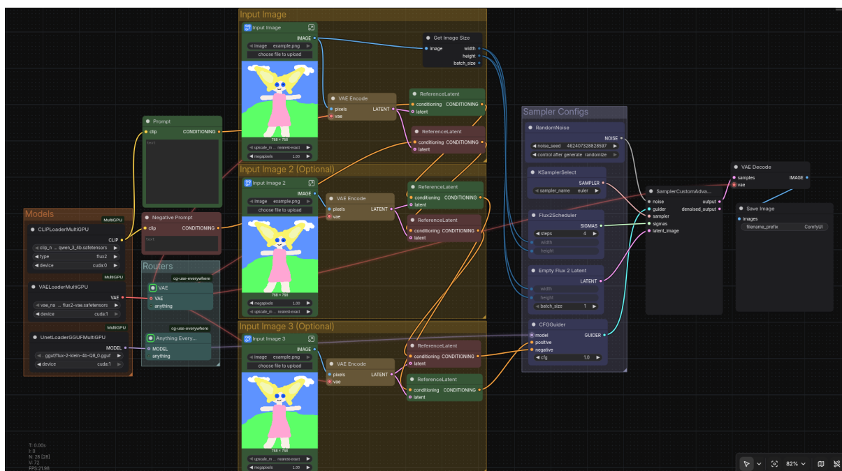
Figure 4.22: Flux2Klein 4B Image Edit Workflow: ComfyUI node graph detailing the generation pipeline, including text conditioning via the Qwen-3 4B text encoder, the DiT-based KSampler, and VAE decoding for photorealistic interior synthesis.
