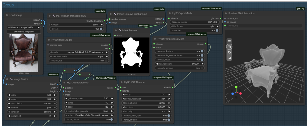
Figure 4.8: 3D Reconstruction Pipeline Part 1: Initial image loading, segmentation (InSpyReNet), and geometry generation via Hunyuan3D DiT.
