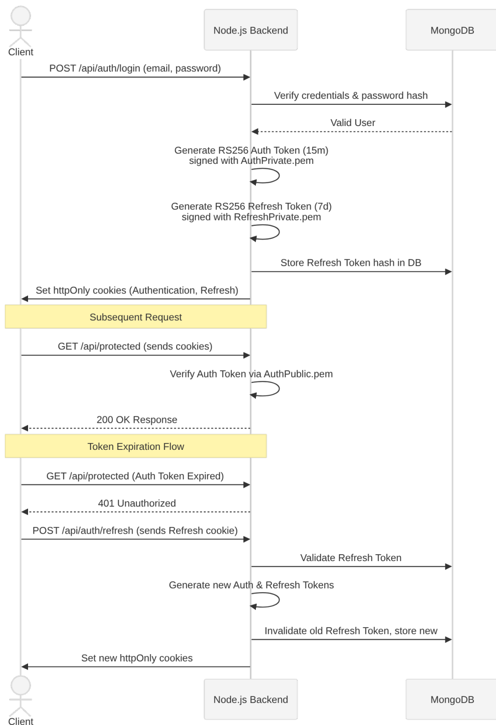
Figure 4.2: JWT Authentication Flow: RS256 token generation, cookie-based session management, and refresh token rotation sequence.
