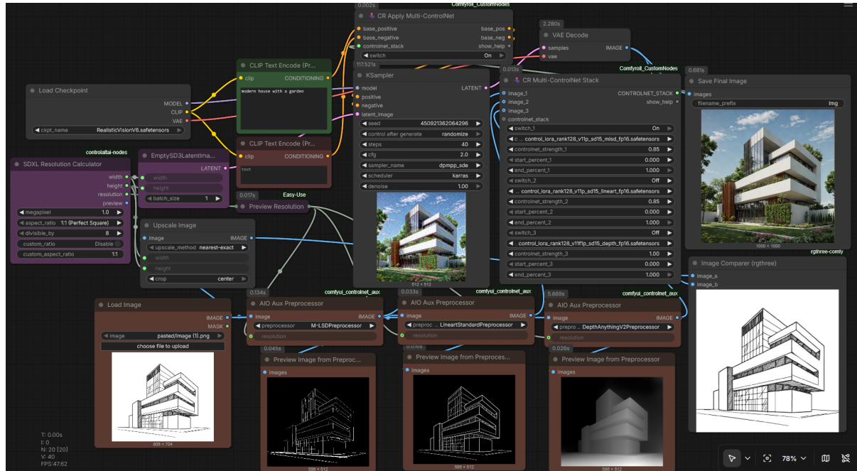
Figure 4.14: Sketch-to-Render Workflow: Tri-layer ControlNet stack (M-LSD, Linear, DepthAnything) converts CAD wireframes into photorealistic renders.
