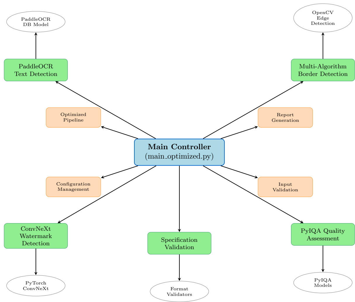
Figure 3: Component Integration and Dependencies
