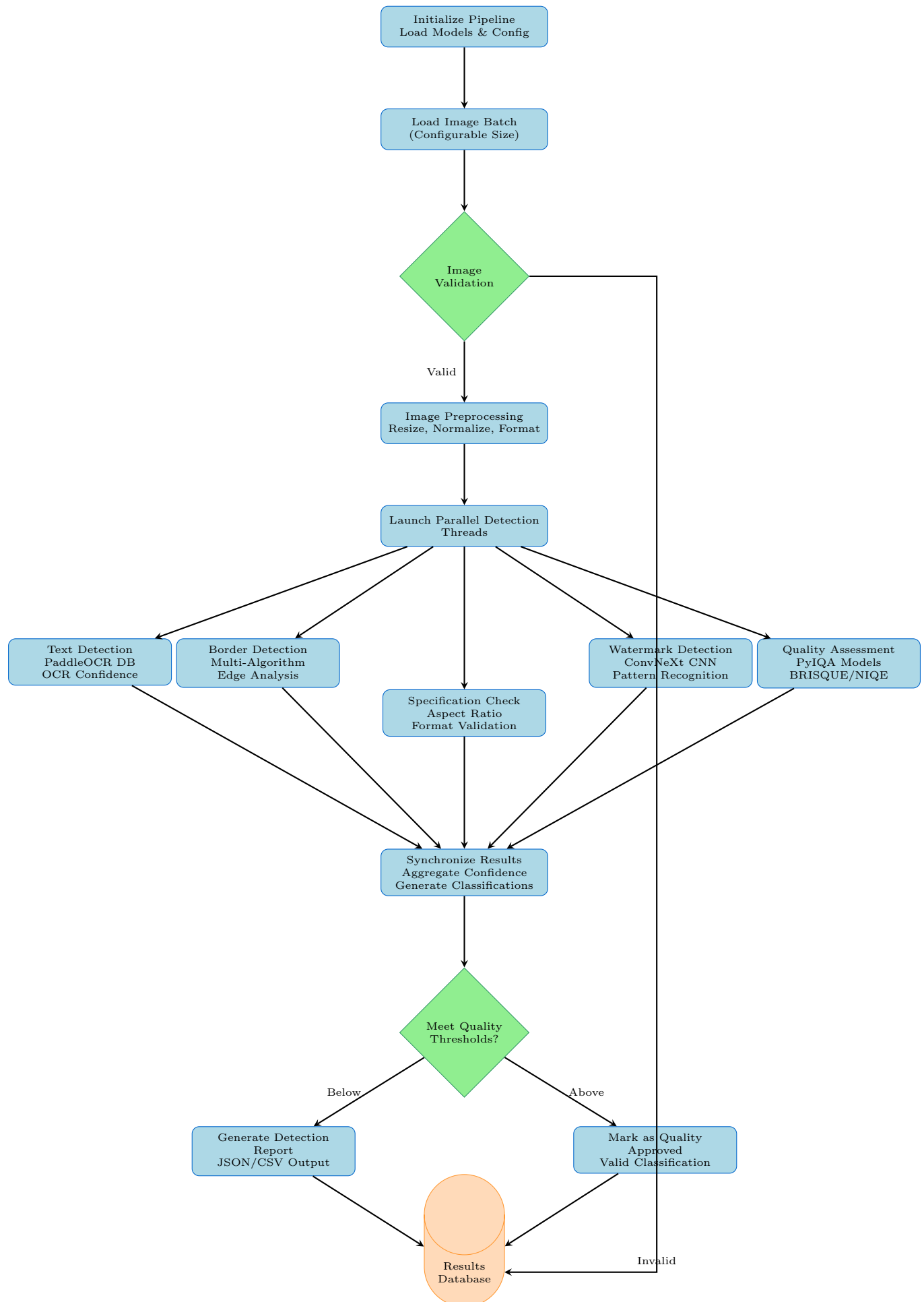
Figure 2: Detailed Pipeline Processing Flow
