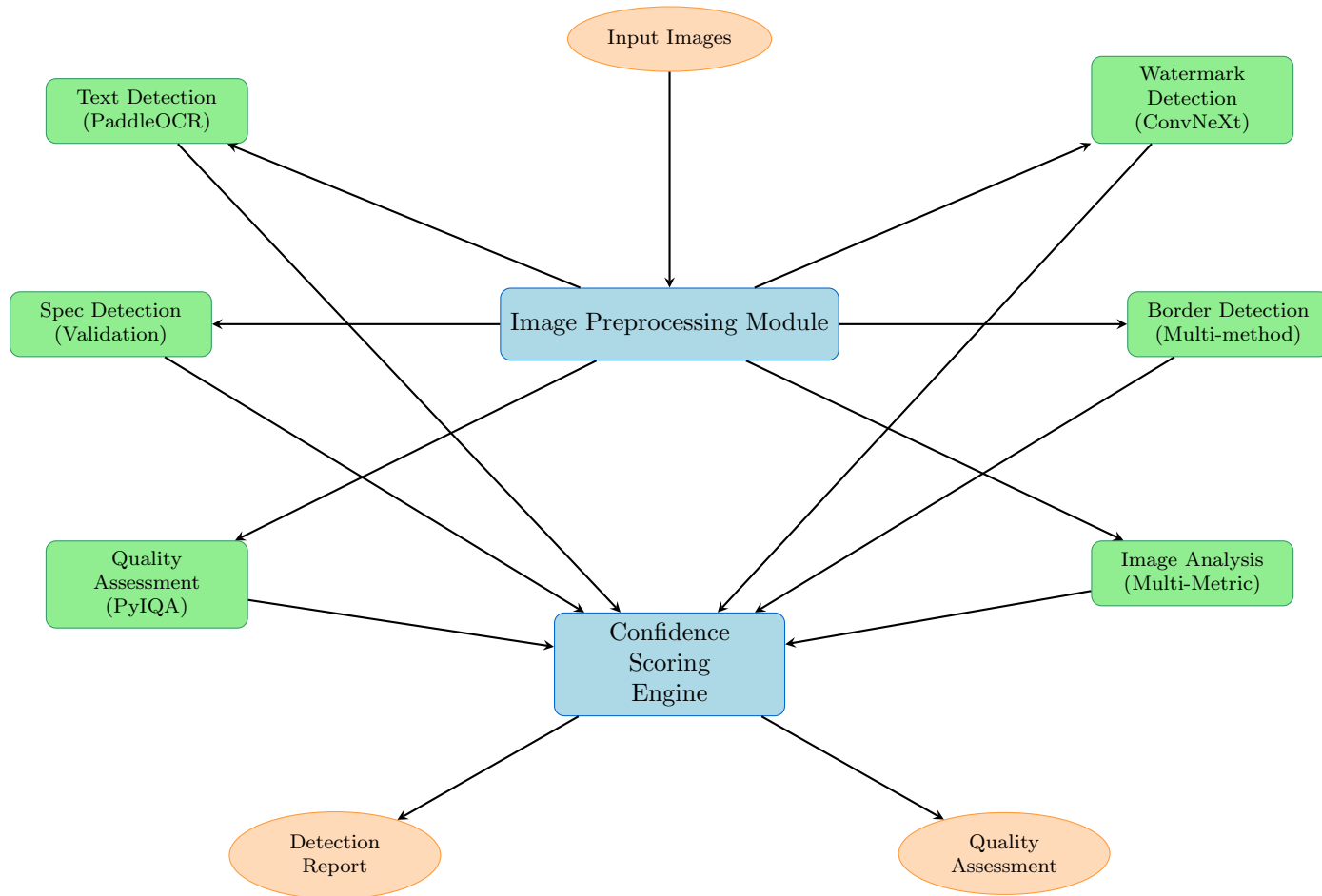
Figure 1: High-Level System Architecture Overview
